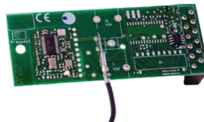
Radio remote control receiver
