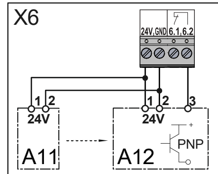
Through photocell A11: Transmitter A12: Receiver
