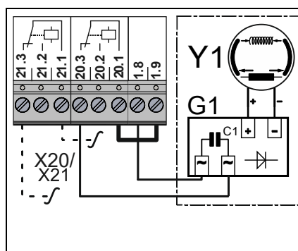
Magnetic brake G1 Rectifier Y1 Magnetic brake
