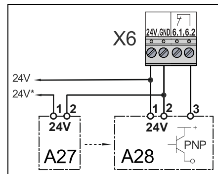
Light curtain A27: Transmitter A28: Receiver
