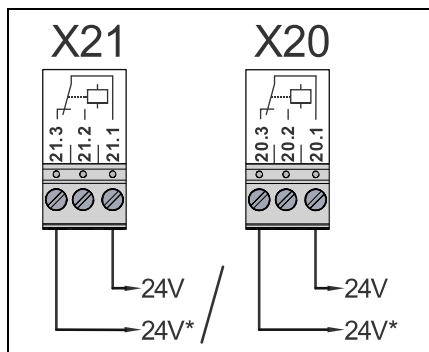
X20: Function relay X21: Function relay (Test light curtain)
